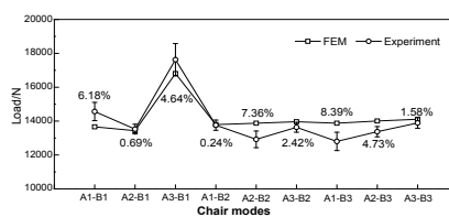
Fig. 13: Comparison between experiment and FEM.
