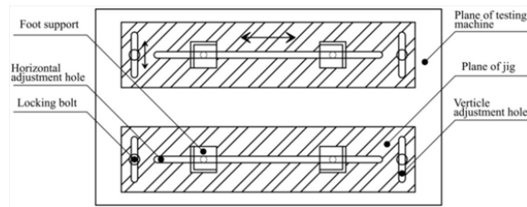
Fig. 1: The diagram of fixture.
