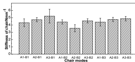
Fig. 9: The stiffness of chair.
