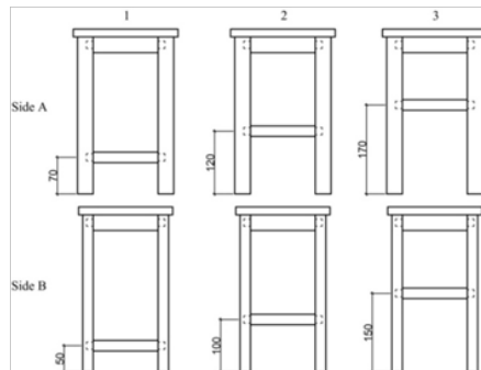
Fig. 4: The varied principle of stretcher.
